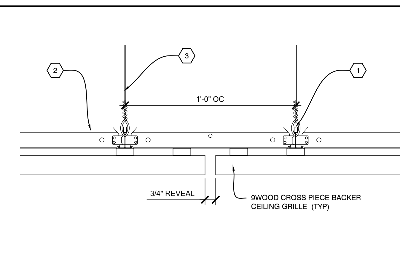
A3 SECTION - ABUTTING REVEAL SCALE: 1/4" = 1'
