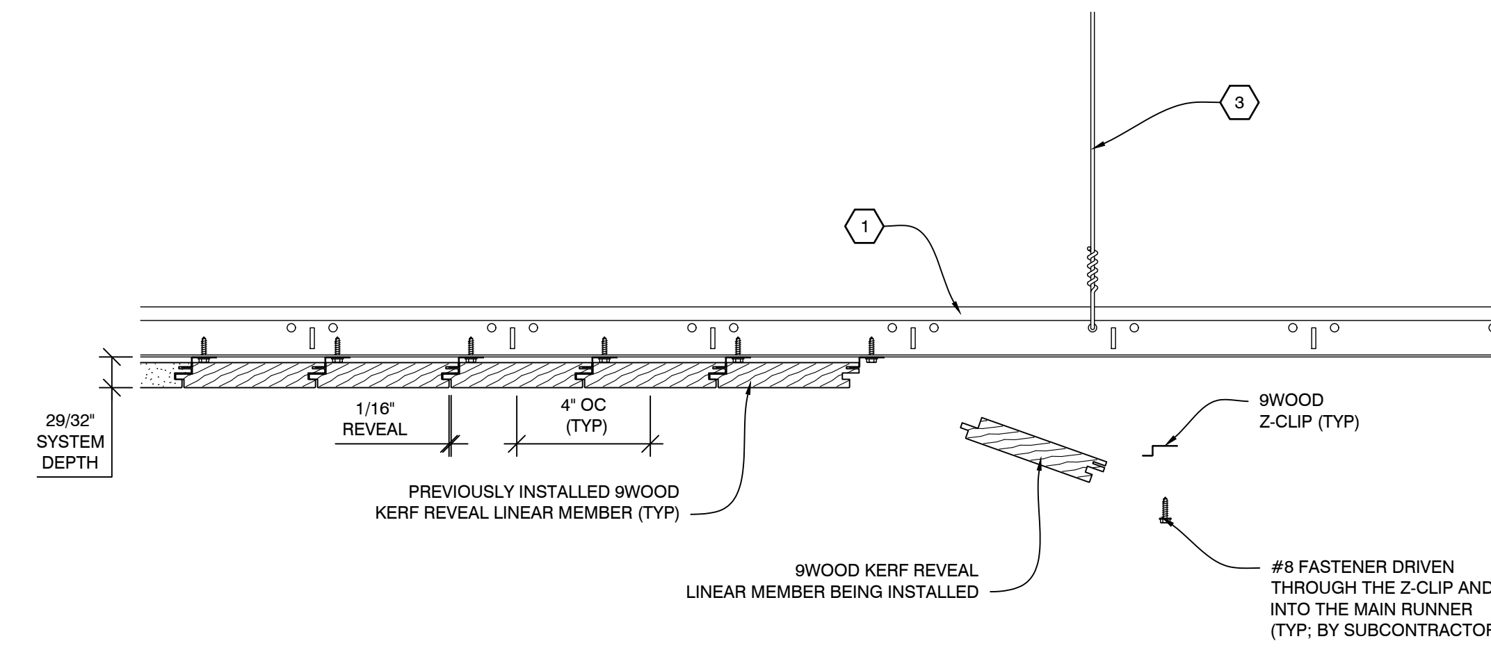
C3 INSTALLATION PROCESS - LINEAR LINEAR WOOD MEMBER SCALE: 1/4" = 1"
