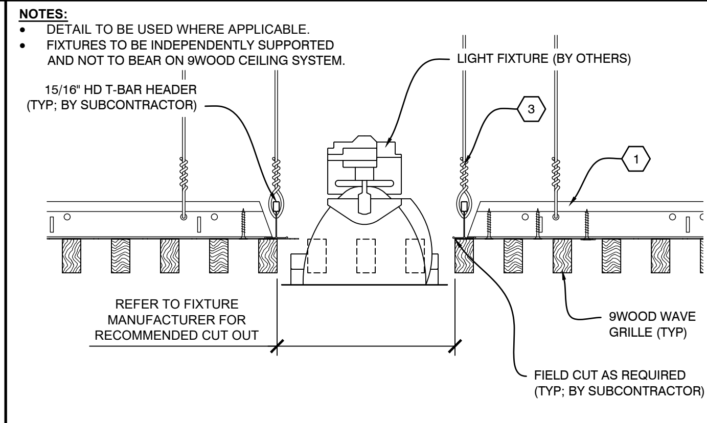
B2 SECTION - LIGHT FIXTURE
