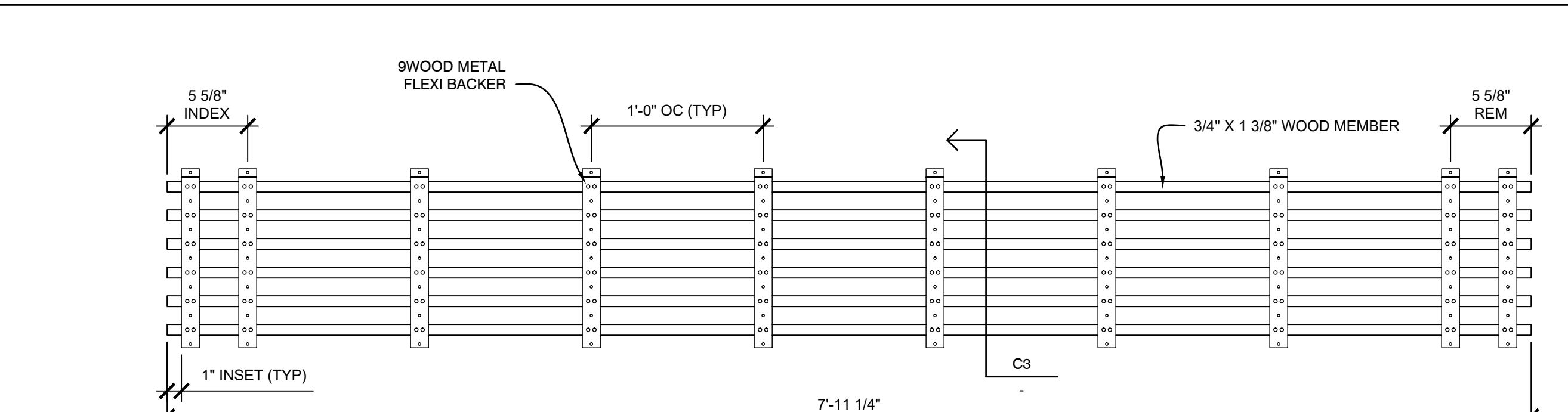
D3 PLAN VIEW - WAVE GRILLE "1.8"
