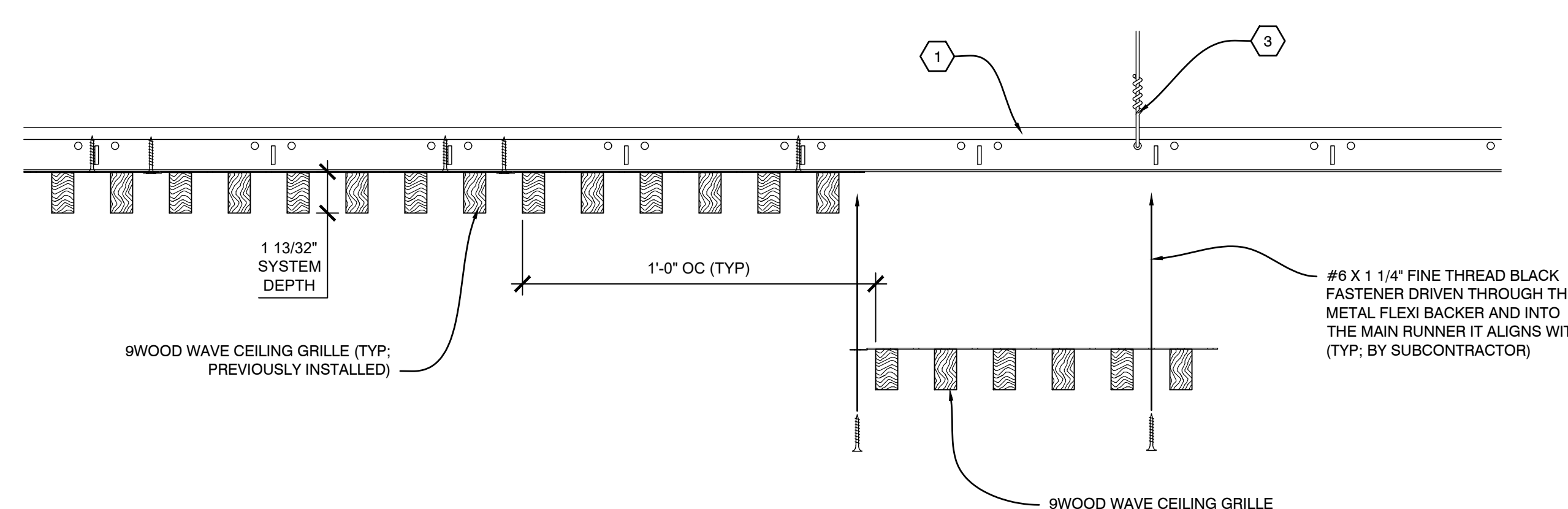
C1 INSTALLATION PROCESS - WAVE GRILLE
