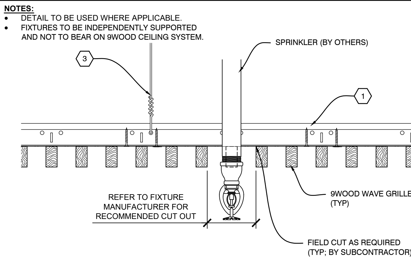
B3 SECTION - SPRINKLER
