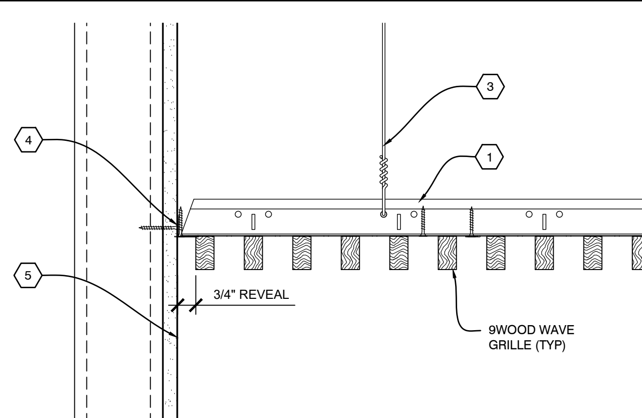
B1 SECTION - PERIMETER
