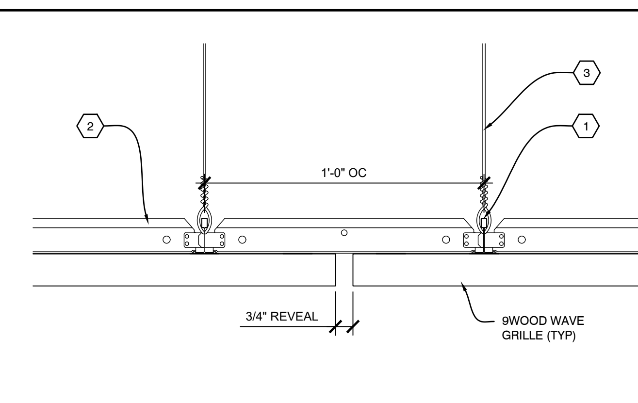
A3 SECTION - ABUTTING REVEAL
