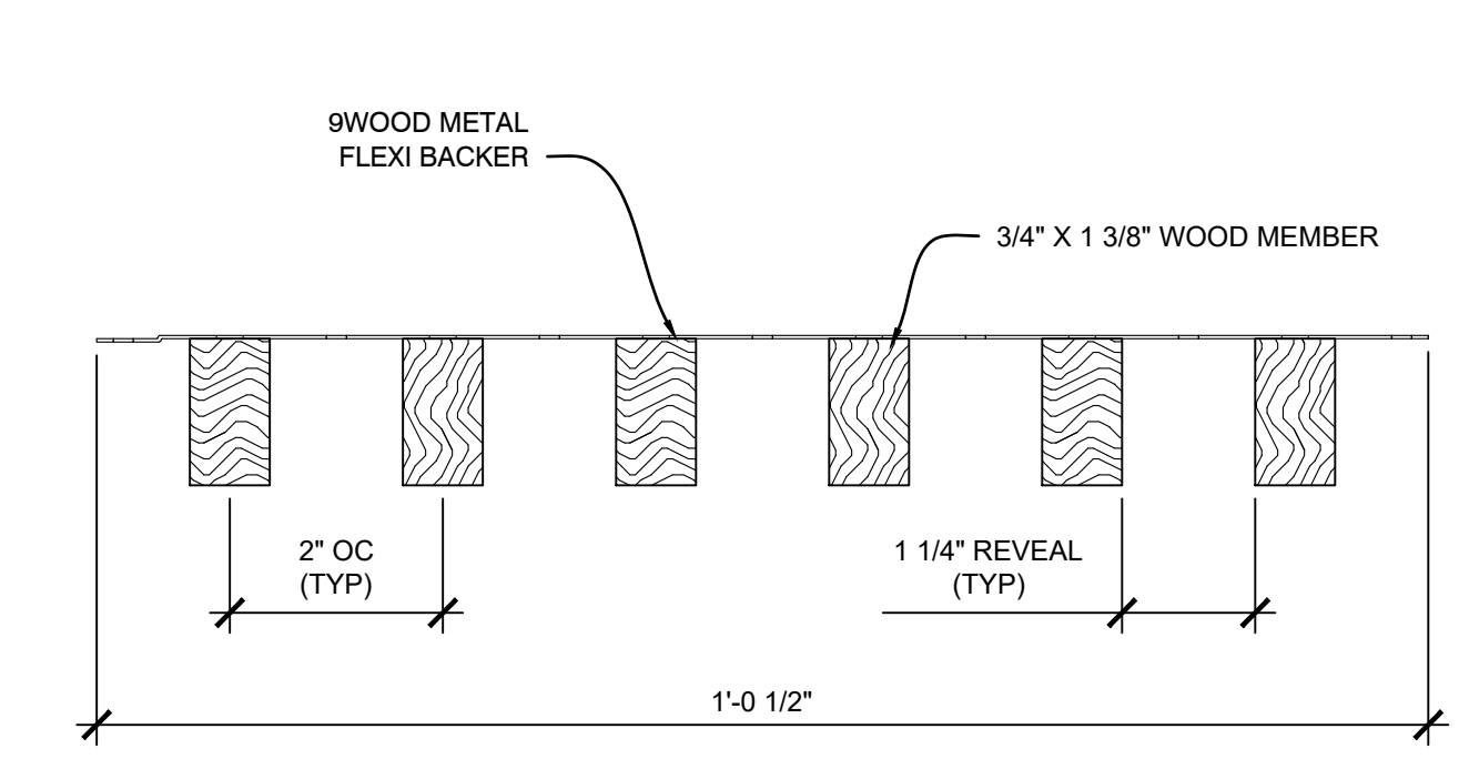
C3 SECTION - WAVE GRILLE
