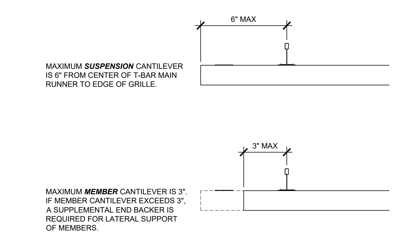
C4 SECTION - CANTILEVER RULES
