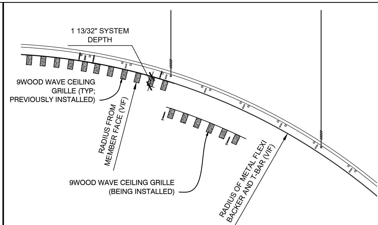
D2 INSTALLATION PROCESS - WAVE GRILLES
