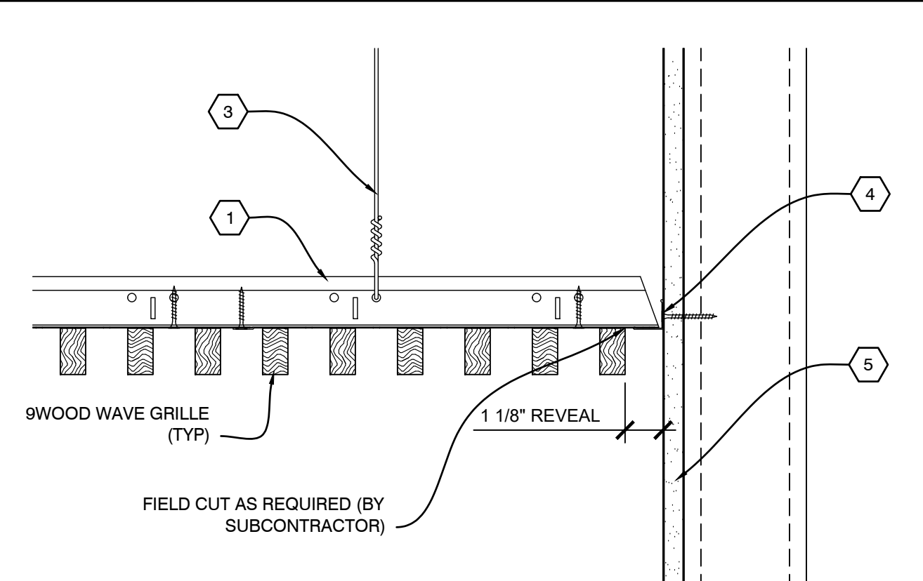
B4 SECTION - PERIMETER
