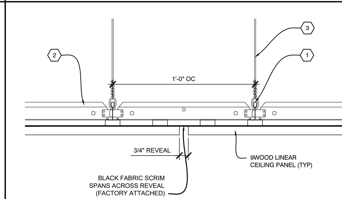
A3 SECTION - ABUTTING REVEAL SCALE: 1/4" = 1'
