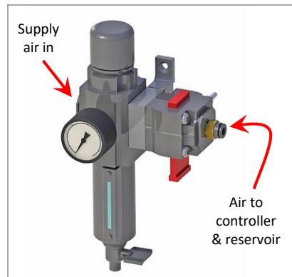
Figure 4. Filter Regulator Connections
