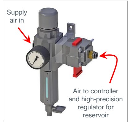
Figure 4. Filter Regulator
