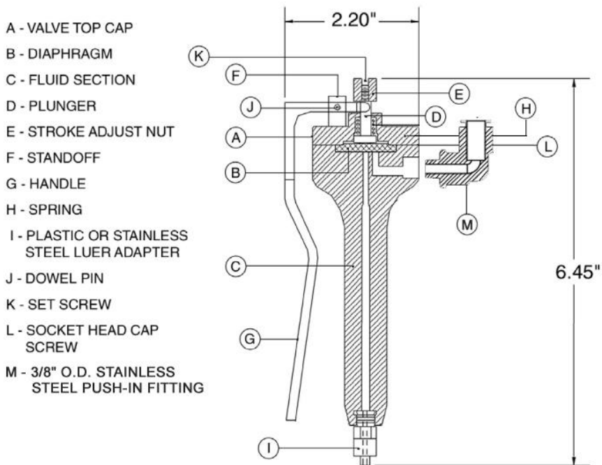
Figure 1. Model 200 Internal Component Diagram
