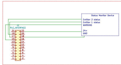
Figure 21. PLC Status Outputs Using Customer-Supplied 24V Source
