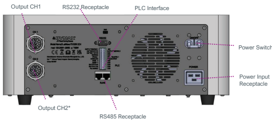
2CH Controller Back Panel
