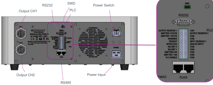
Figure 9. Controller Connections
