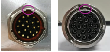
Figure 14. Key (Left) and Keyway (Right)
