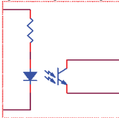
Status Monitor Device Option 2: Optical Coupler
