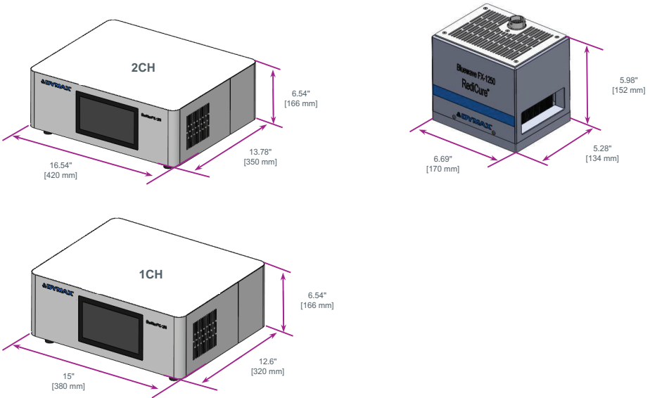
Figure 40. Dimensions
