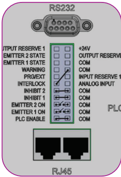
Figure 15. Plug Foot Switch into Controller
