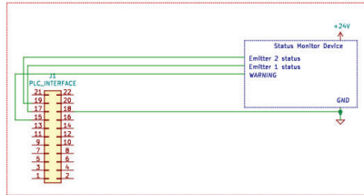
Figure 21. PLC Status Outputs Using Customer-Supplied 24V Source
