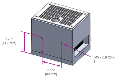
Figure 41. Mounting Hole Locations and Size
