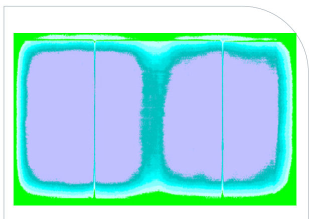
Figure 5. Uniformity of Two Emitters Side-by-Side
