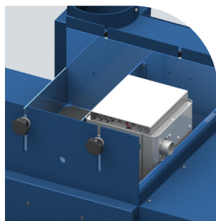
One 5000-EC lamp center mounted 6" wide single exposure
