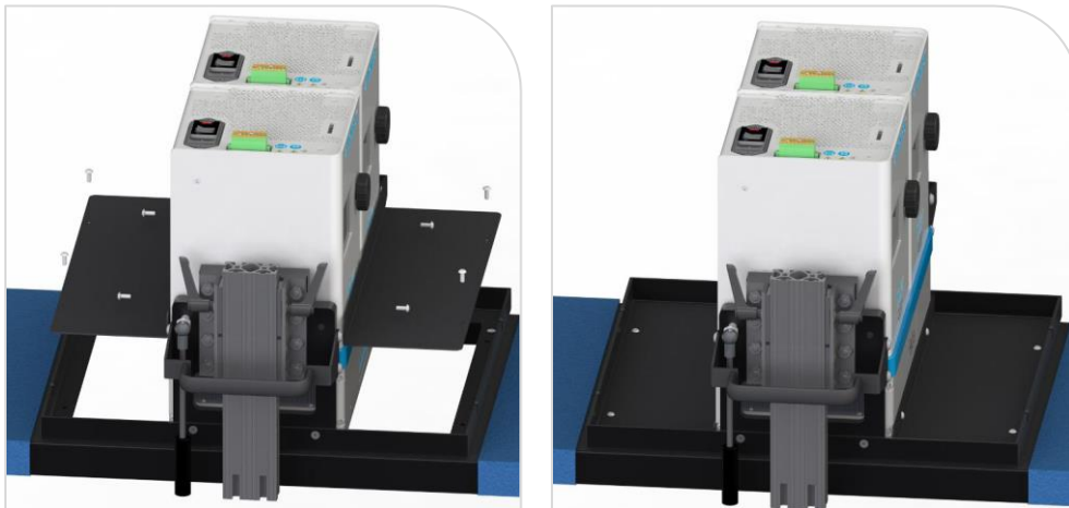
Figure 15. Attach Emitter to Plates
