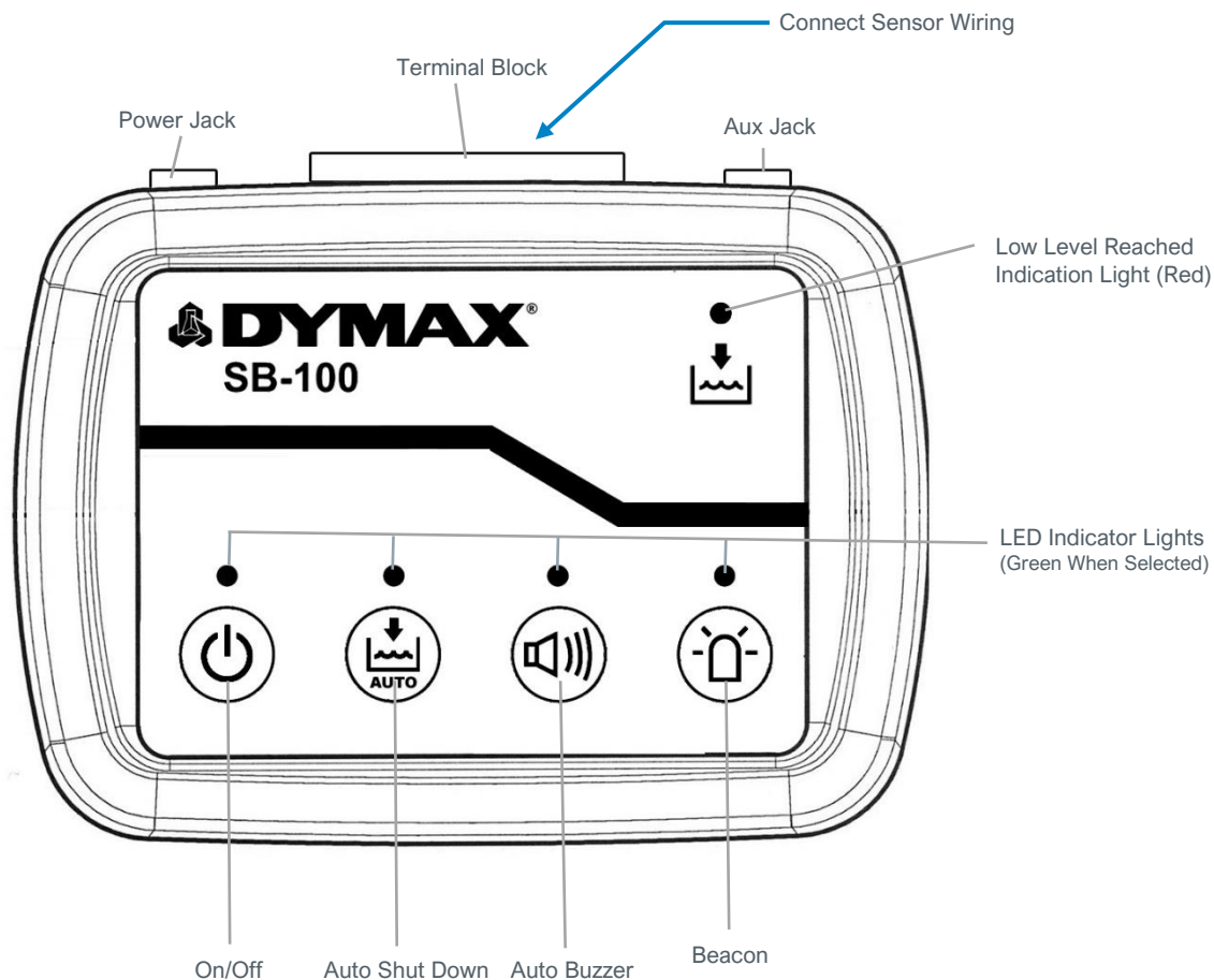
Figure 1. SB-100 Controller
