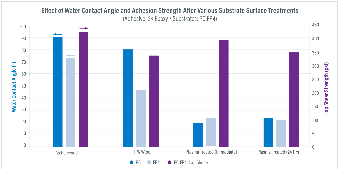
Graph 8. Contact angle (left) and adhesion strength (right) for PC to FR-4 (2K epoxy)
