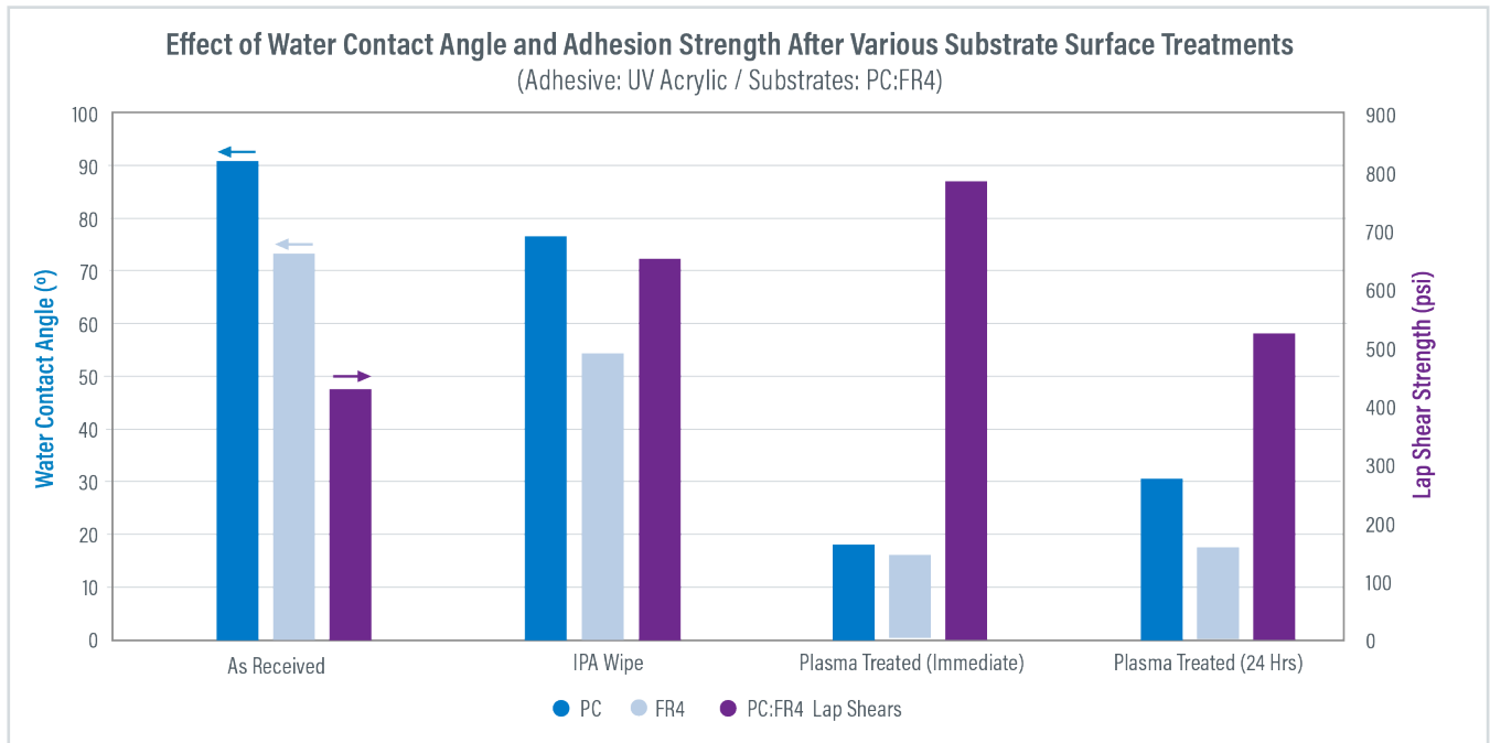
Graph 5. Contact angle (left) and adhesion strength (right) for PC to FR-4 (UV-curable acrylic)
