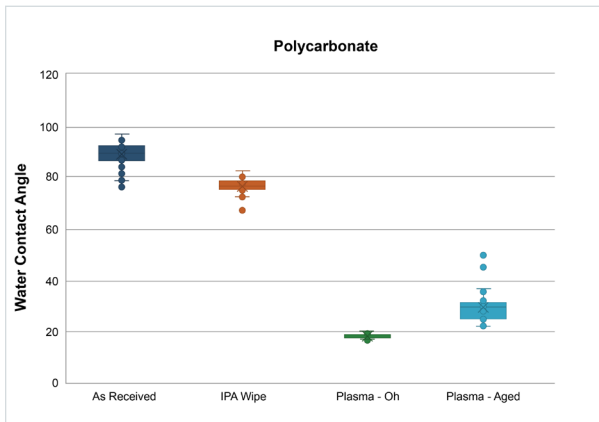
Graph 3. Polycarbonate contact angles by surface preparation method
