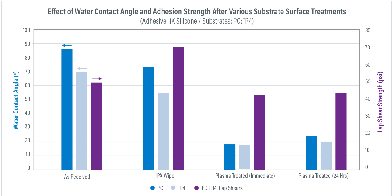
Graph 7. Contact angle (left) and adhesion strength (right) for PC to FR-4 (RTV silicone)
