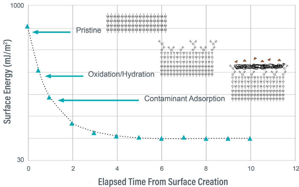
Graph 2. Surface energy decay of a freshly cleaned metal (no time scale is included because reaction rates depend on the environment)
