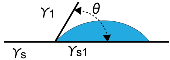
Figure 2. Contact Angle ( \theta ) is determined by the balance of interfacial energies: liquid surface tension \gamma_l , solid surface energy \gamma_s , and the remaining interfacial energy \gamma_{sl}
