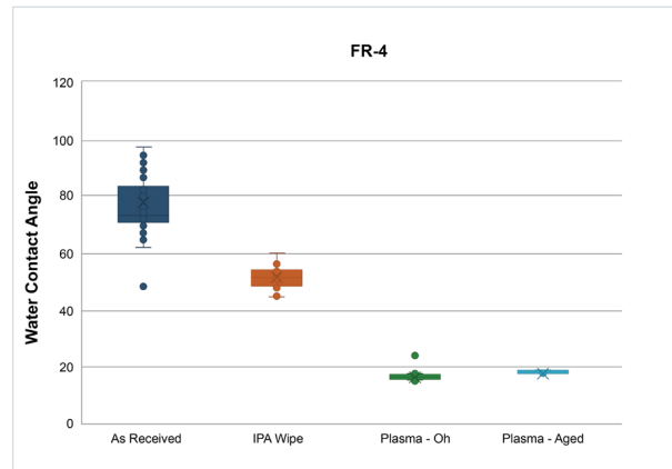
Graph 4. FR-4 contact angles by surface preparation method
