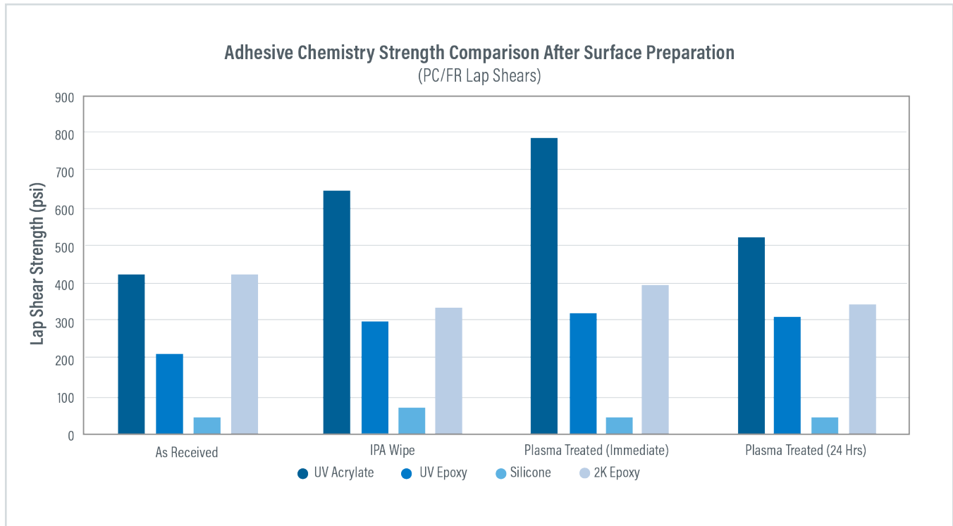
Graph 9. Consolidated Summary - Adhesion strength by surface preparation method
