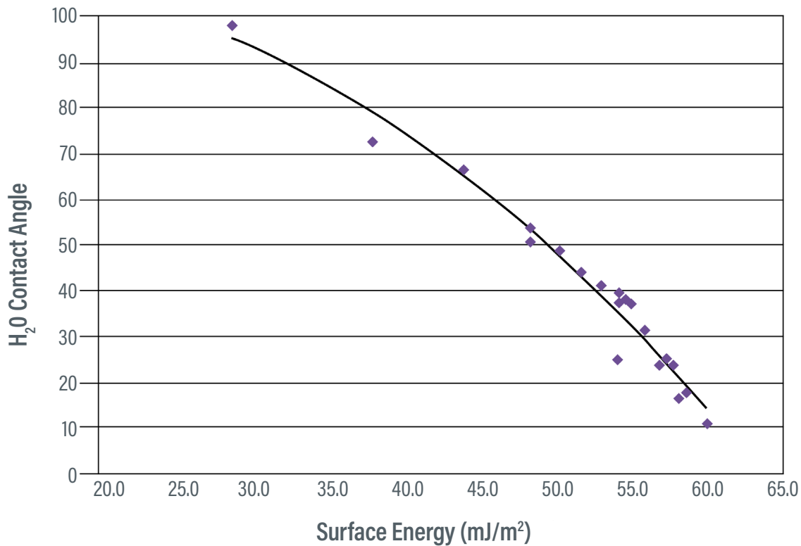
Graph 1. Surface Energy vs. Water Contact Angle
