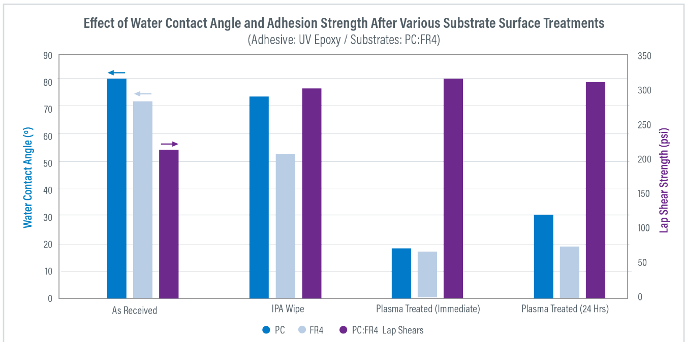
Graph 6. Contact angle (left) and adhesion strength (right) for PC to FR-4 (UV-curable epoxy)
