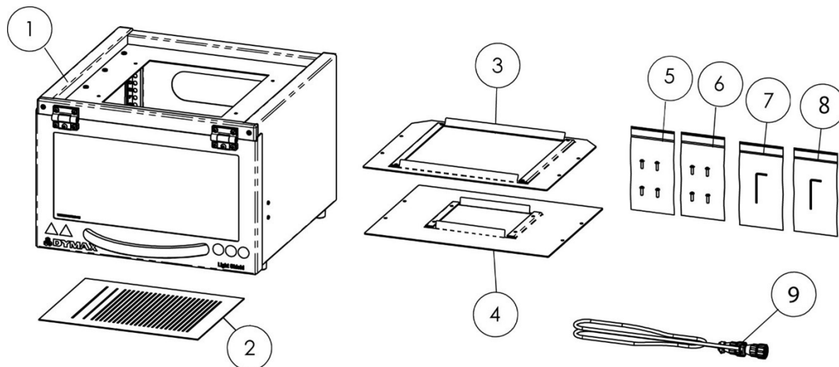
Figure 2. Light Shield (PN 41175) Components
