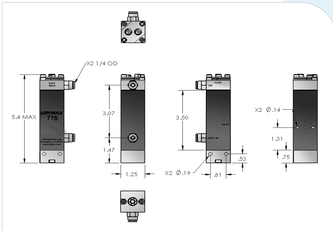
Figure 1. Model 775 Dimensions
