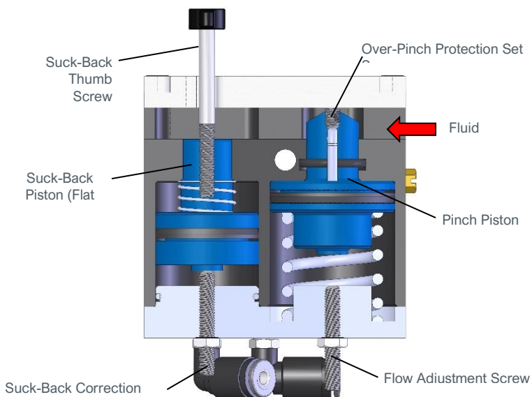
Figure 6. Model 830 Cross Section (Flow from Right to Left)
