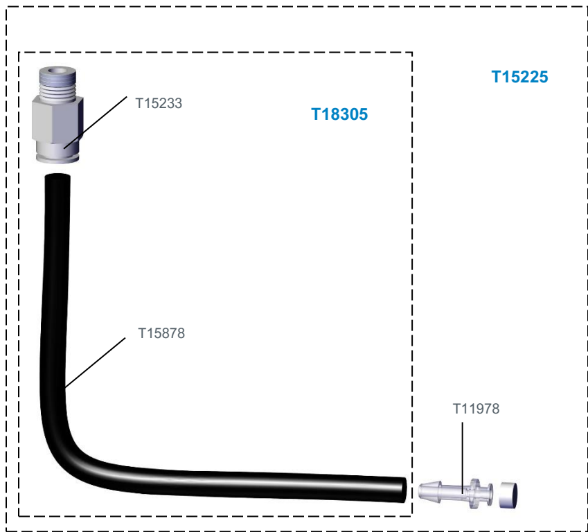
Figure 14. Tubing Assembly
