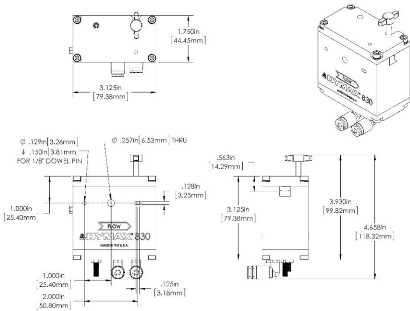
Figure 15. Dimensions
