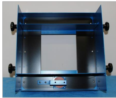
Figure 46. Lamp Brackets & RF Detector Support
