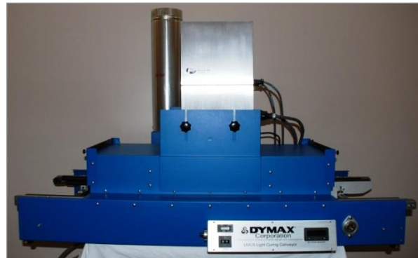
Figure 3. Conveyor with Fusion Lamps Installed
