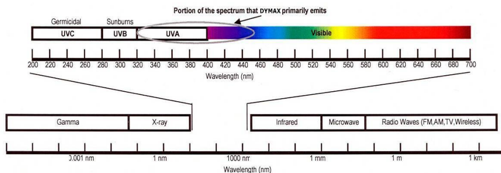
Figure 1. UV Spectrum
