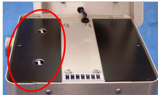
Figure 9. Add Second Temperature Control Plate
