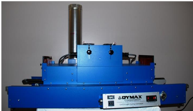
Figure 2. Conveyor with Dymax Lamps Installed
