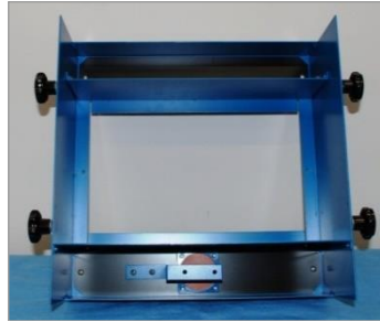
Figure 43. Install Spacers & RF Detector Support
