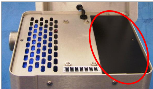
Figure 8. Add First Temperature Control Plate
