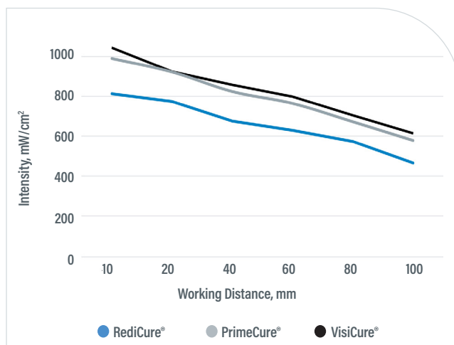
Figure 3. BlueWave® AX-550 V2.0 Emitter Relative Intensity vs. Distance
