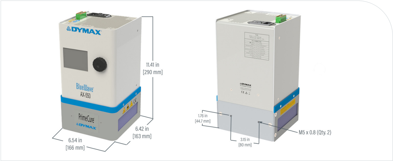
Figure 1. BlueWave® AX-550 V2.0 Dimensions
