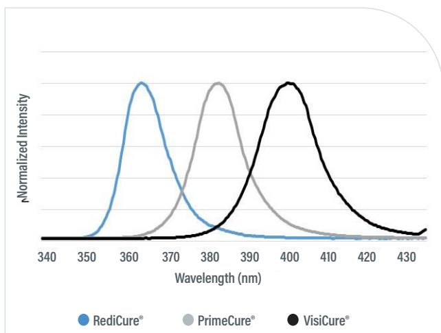
Figure 2. BlueWave® AX-550 V2.0 Emitter Spectral Output Chart
