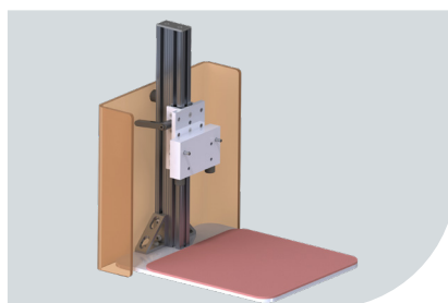
Mounting Stand with Acrylic Back Shield
