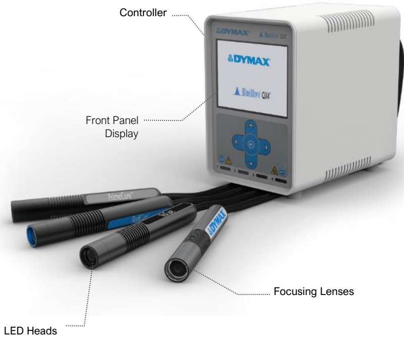
Figure 2. Main Components of a BlueWave QX4
