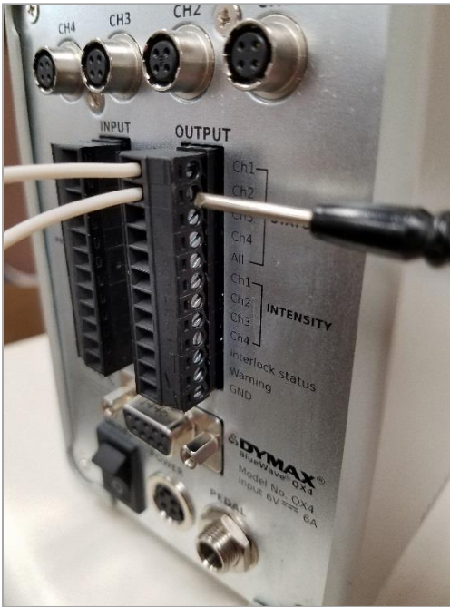
Figure 30. PLC Wire Attachment, Terminals Installed
