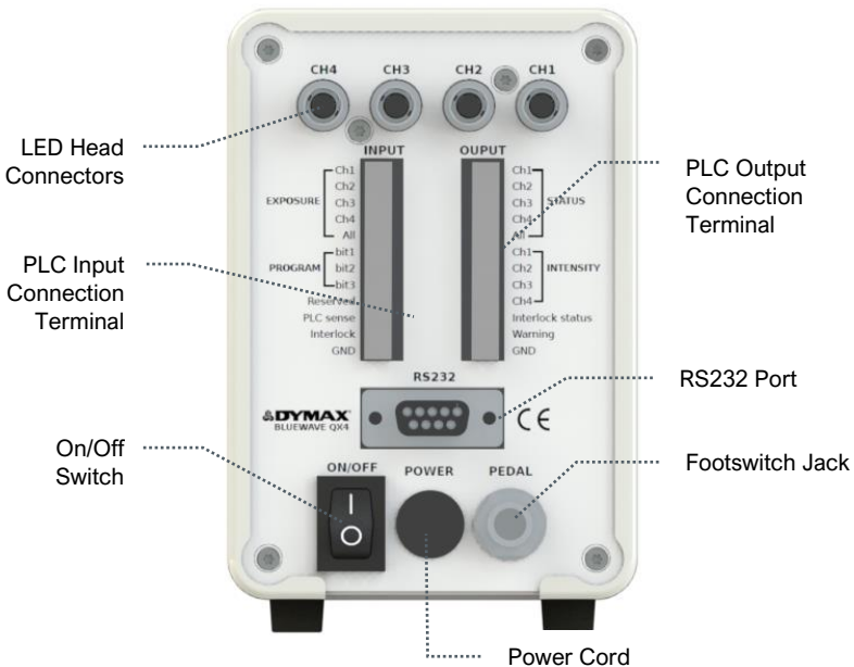
Figure 4. Back Panel Controls & Connections
