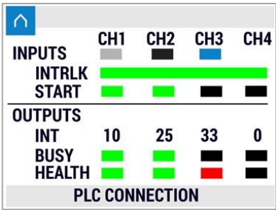
Figure 25. PLC Mode Screen
