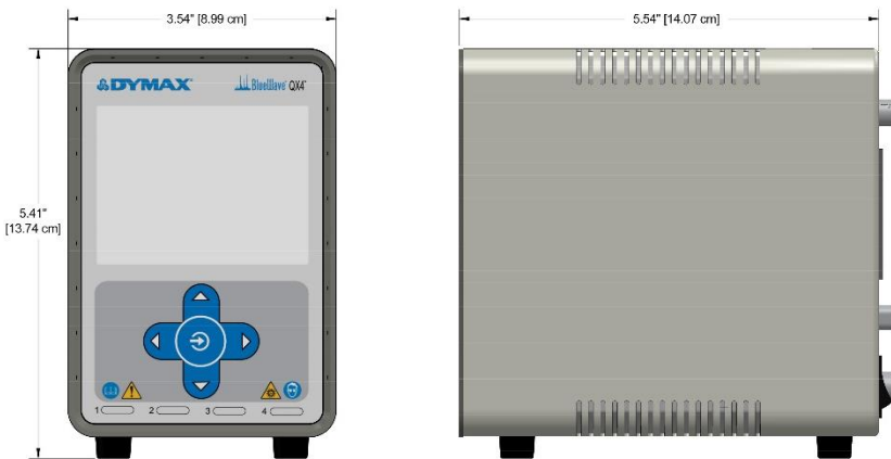
Figure 45. Dimensions - Controller
