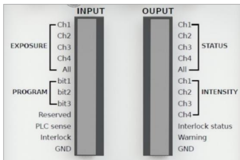
Figure 32. PLC Inputs & Outputs
