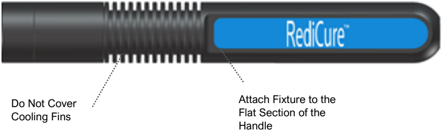
Figure 8. Fixturing Recommendations
