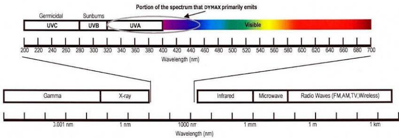
Figure 1. UV Spectrum
