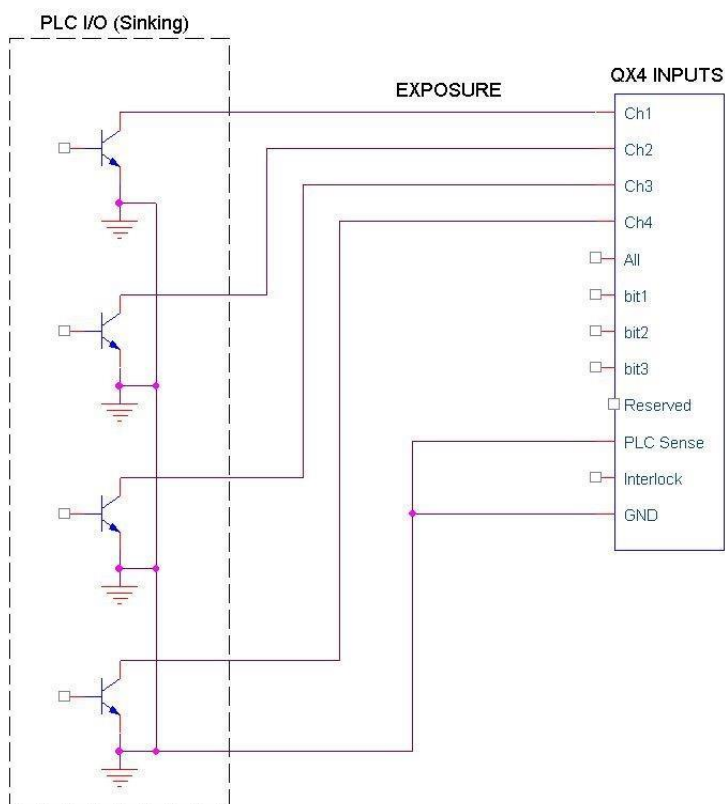
Figure 33. Connection Diagram
