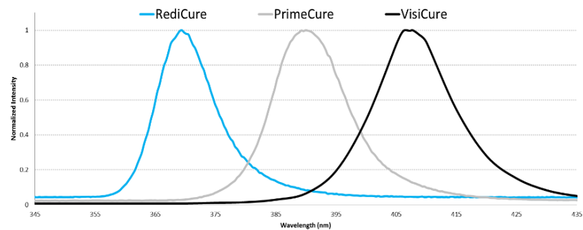
Figure 43. BlueWave QX4 Spectral Output
