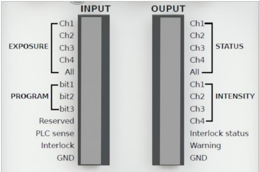
Figure 26. PLC Inputs & Outputs
