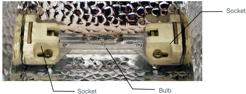
Figure 9. Flood Lamp Bulb Installed
