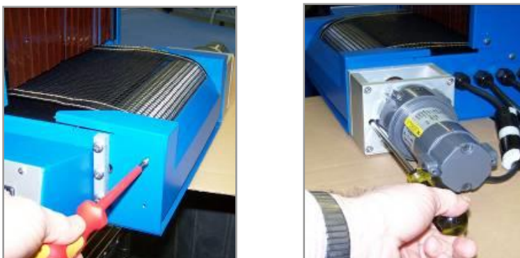
Figure 35. Installing Pinch Guard (front & back)
