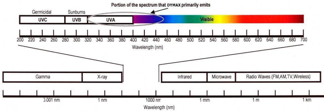
Figure 1. UV Spectrum
