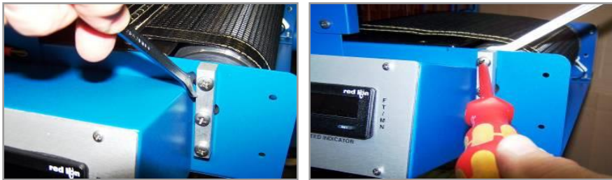
Figure 34. Tightening Drive-Roller Shaft-Support Fasteners
