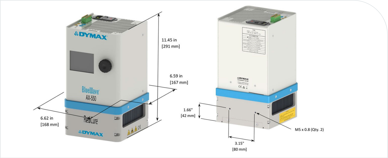
Figure 1. BlueWave® AX-550 Dimensions
