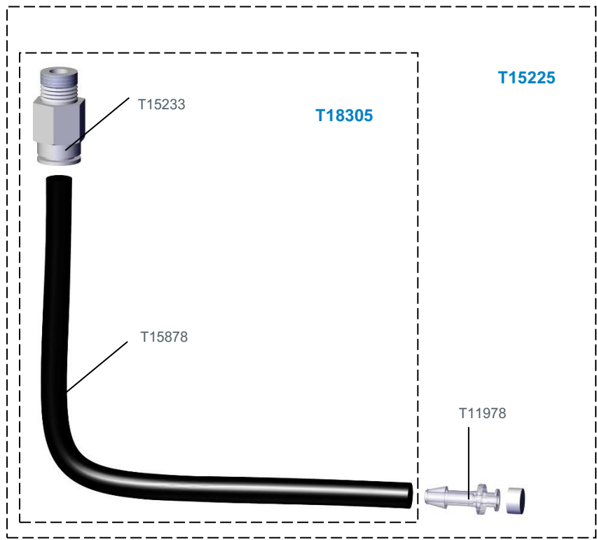
Figure 14. Tubing Assembly
