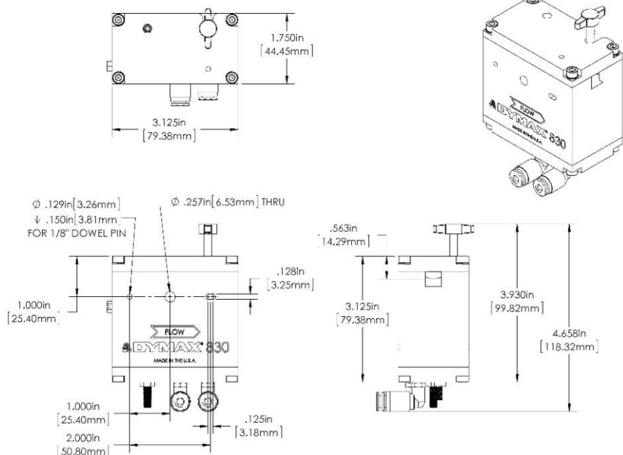
Figure 15. Dimensions
