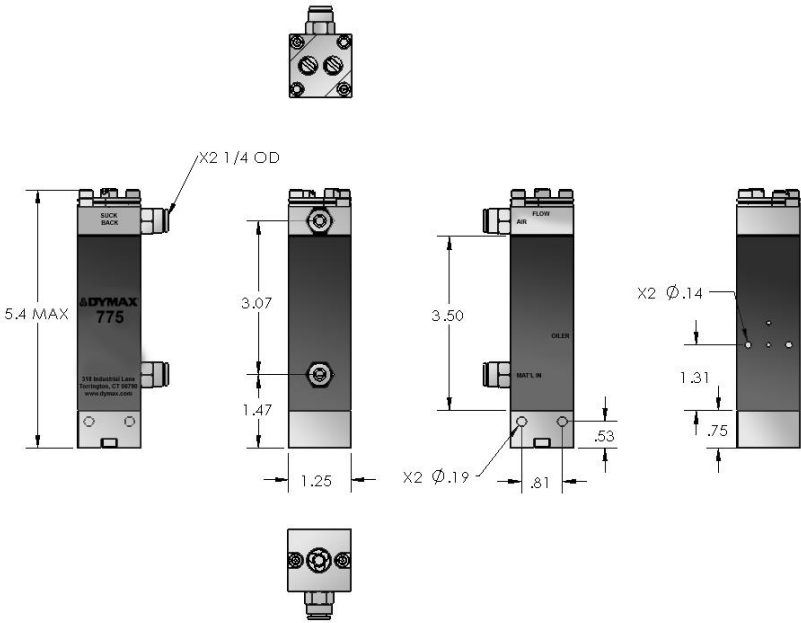
Figure 6. Model 775 Dimensional Drawing
