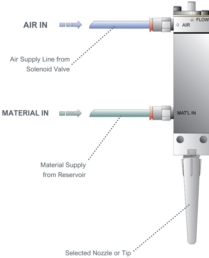
Figure 3. Model 775 Interconnect Diagram
