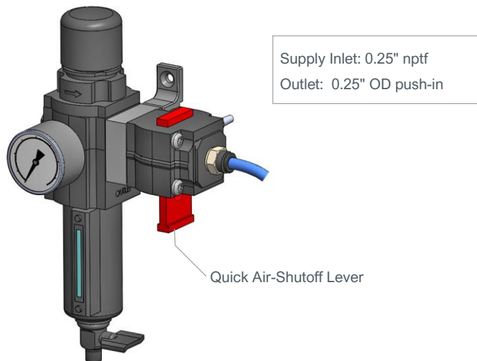
Figure 13. Air Filter/Regulator with Quick Air-Shutoff Lever (PN T16307)
