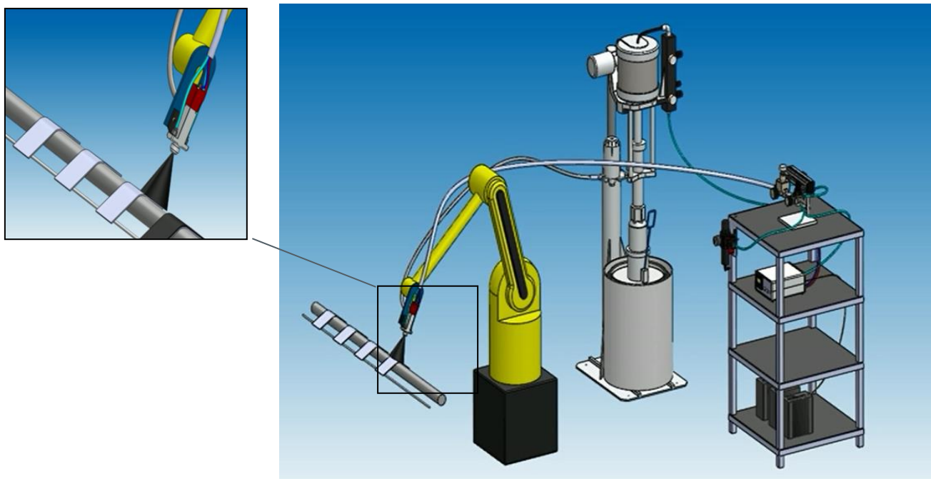
Figure 15. Robotic System
