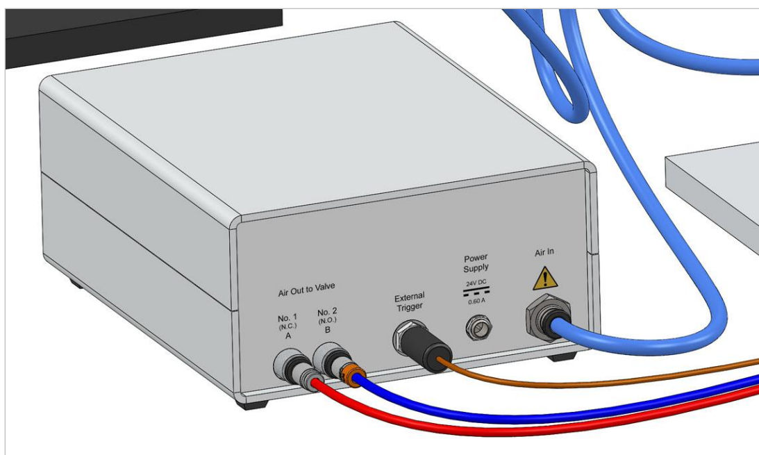
Figure 7. DVC-345 Connections
