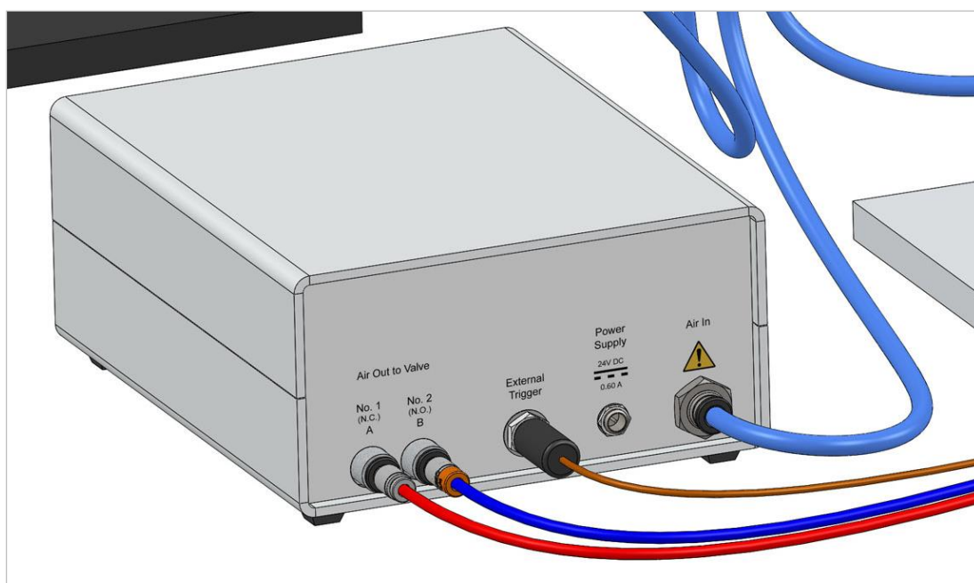
Figure 7. DVC-345 Connections
