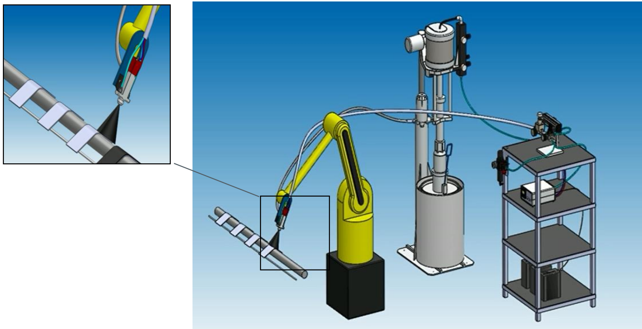
Figure 15. Robotic System
