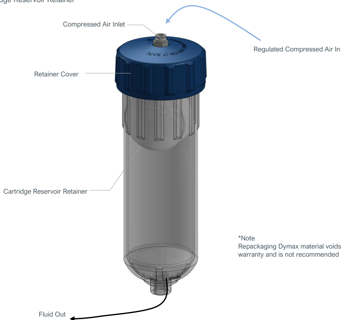
Figure 2. Cartridge Reservoir Retainer
