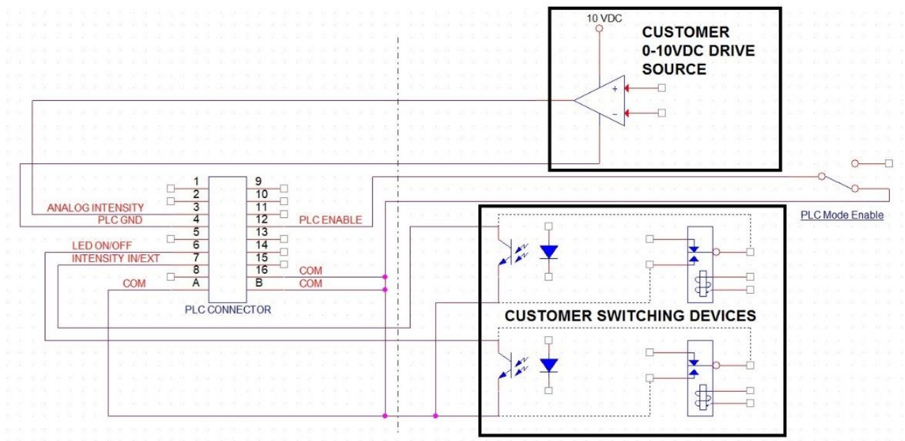
Figure 19. PLC Connection
