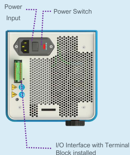
Figure 7. Controller, Topside
