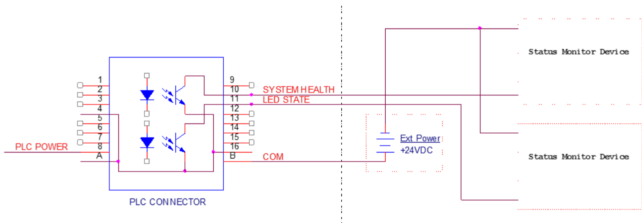
Figure 21. PLC Status Outputs Using Customer-Supplied 24V Source
