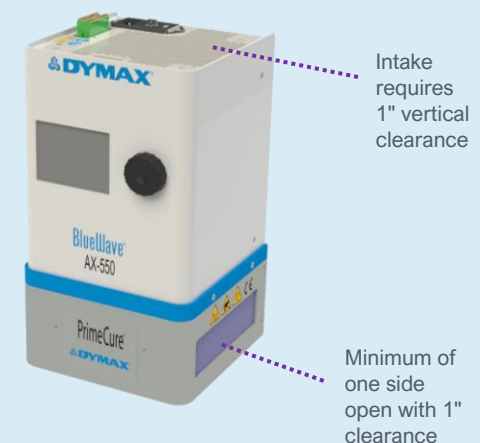
Figure 6. Minimum Clearance
