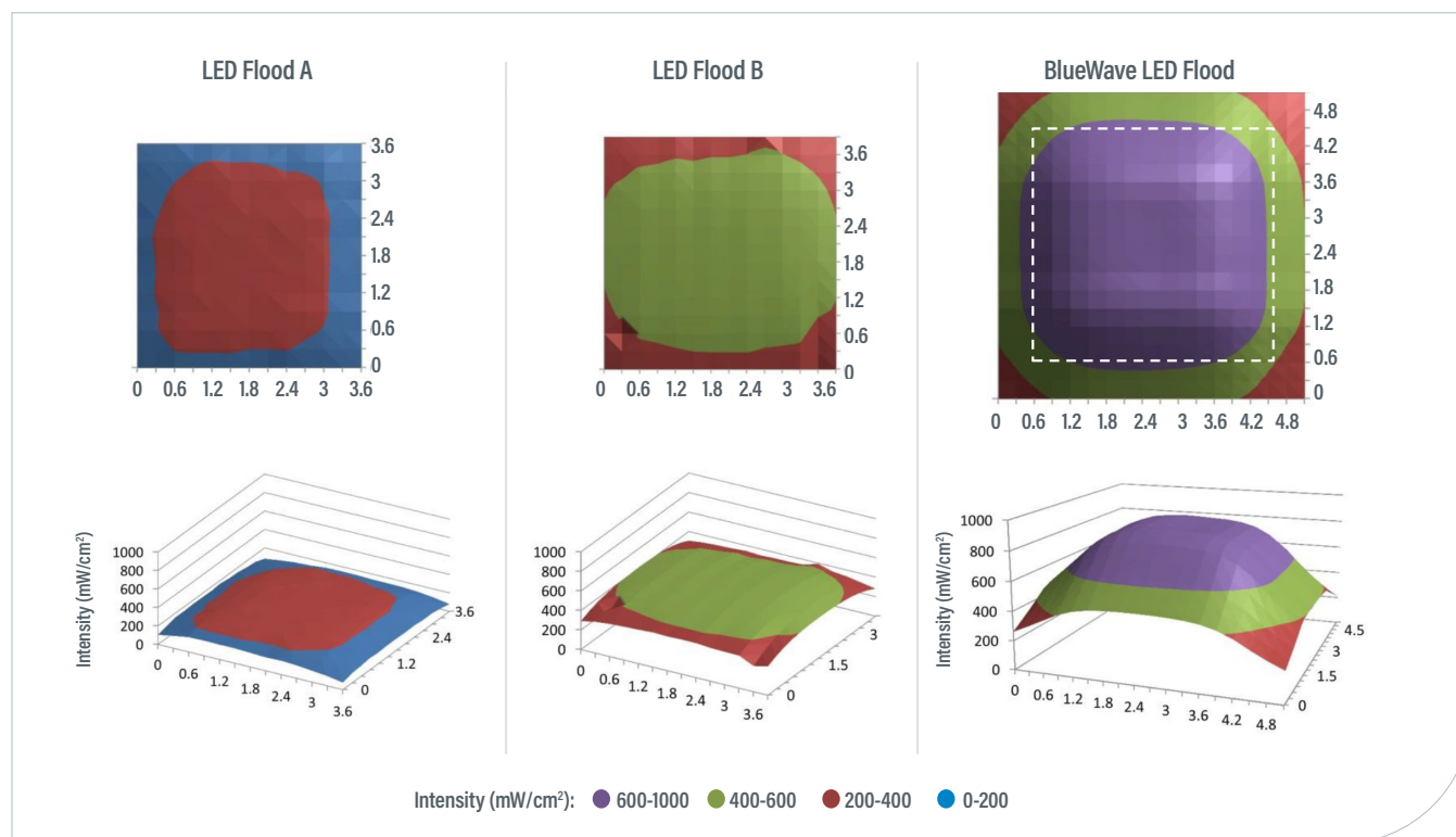
Figure 2. Curing Uniformity
