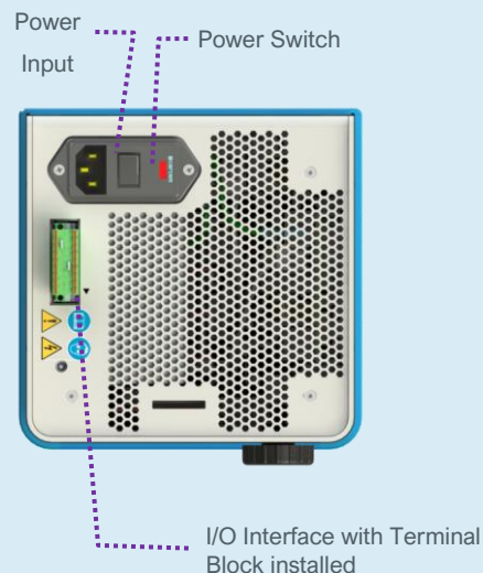
Figure 7. Controller, Topside
