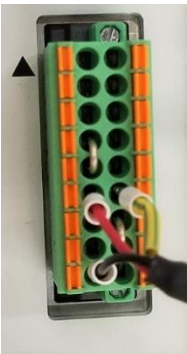
Figure 17. Foot Switch Wiring Pin Locations
