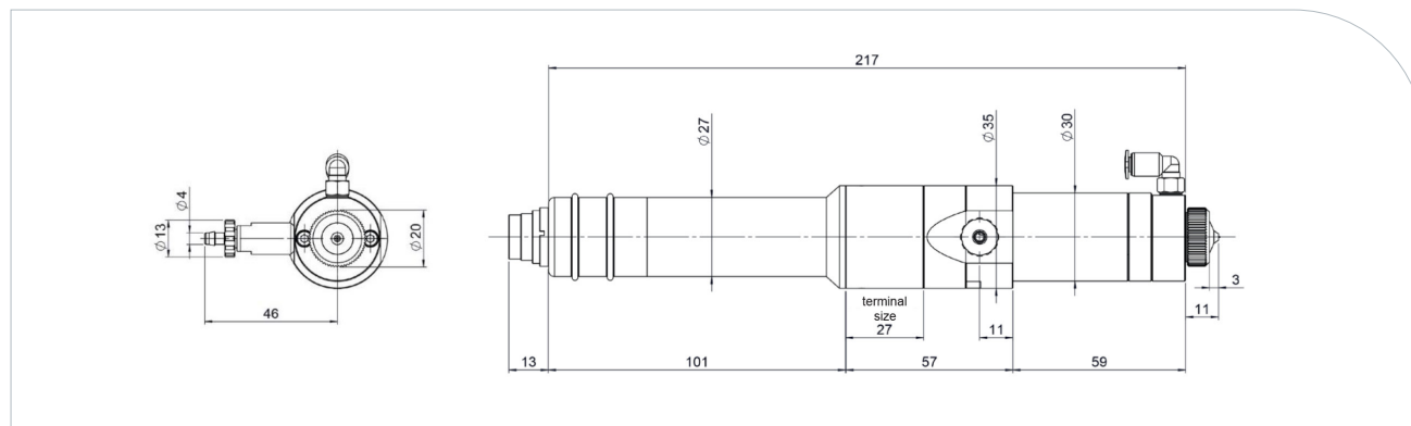
Figure 1. eco-SPRAY Dimensions
