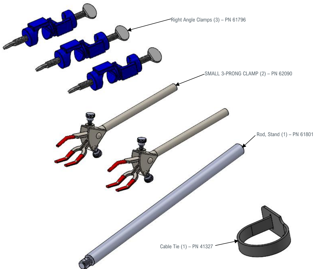
Figure 1. Lightguide Stand Expansion Kit (PN 41595)
