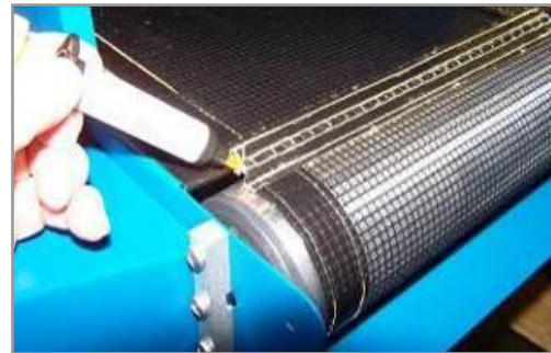
Figure 22. Applying Adhesive
