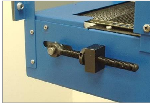
Figure 15. Belt-Tension Adjustment Knob
