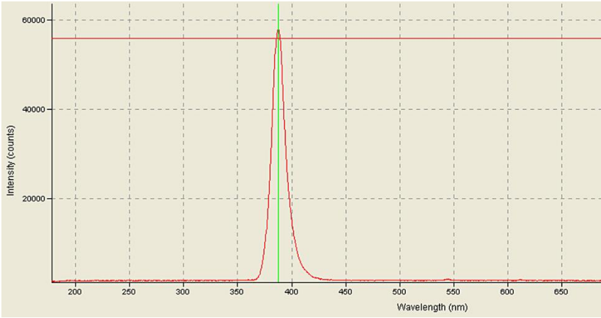
Figure 30. PrimeCure Wavelength
