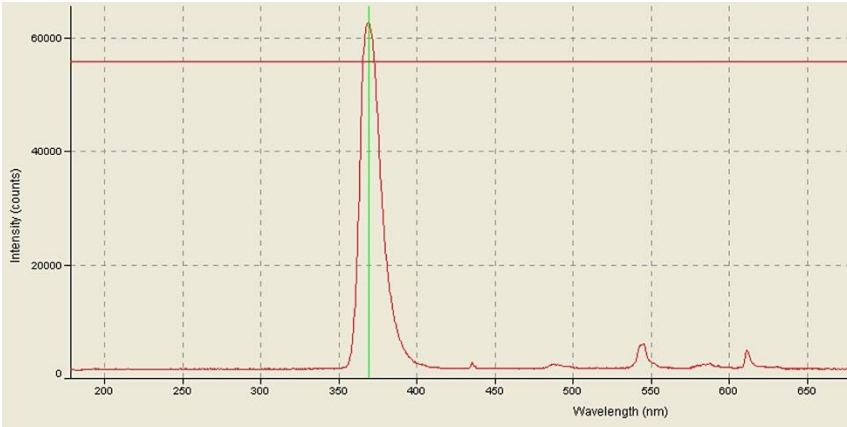
Figure 32. RediCure Wavelength
