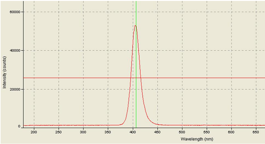
Figure 31. VisiCure Wavelength
