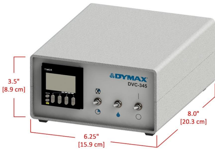
Figure 5. Controller Dimensions
