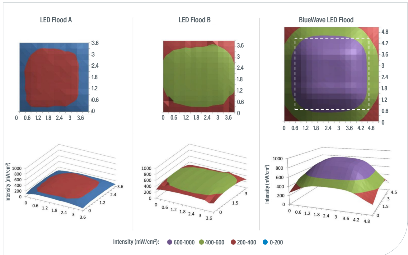
Figure 2. Curing Uniformity
