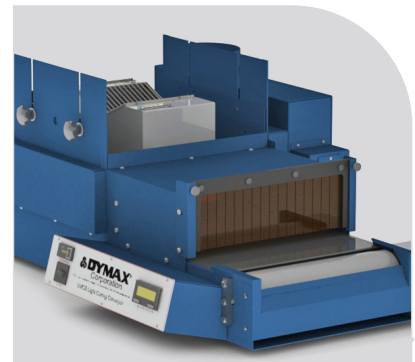
Two LED Floods Mounted in a UVCS Conveyor
