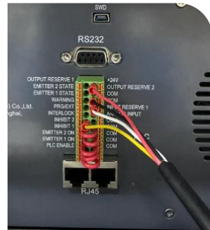
Controller PLC Socket
