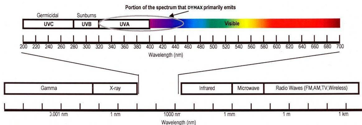
Figure 1. UV Spectrum
