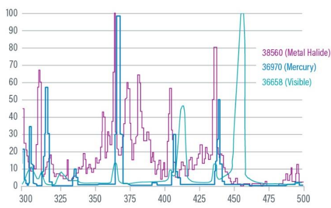
Figure 13. Spectral Outputs for Dymax 400-Watt Flood Bulbs
