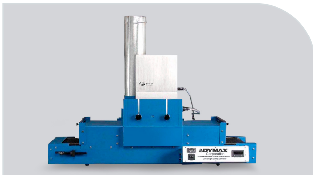
UVCS conveyor with one center-mounted Fusion
