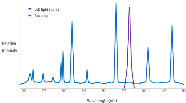
Figure 2. Various adhesive bond-performance results when cured with a conventional arc lamp and LED light sources
