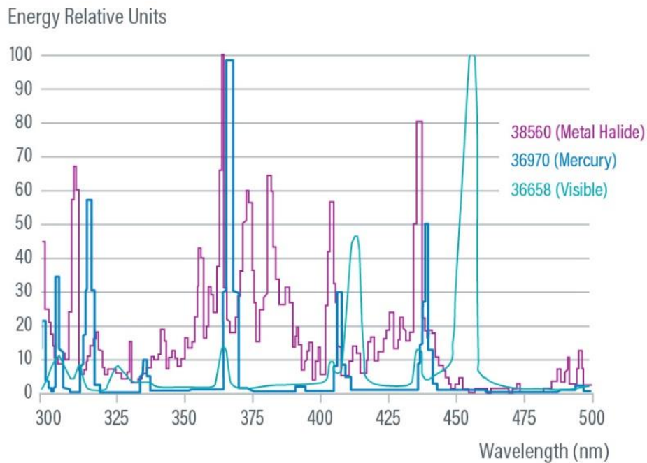
Figure 36. ECE Flood Lamp Spectral Output
