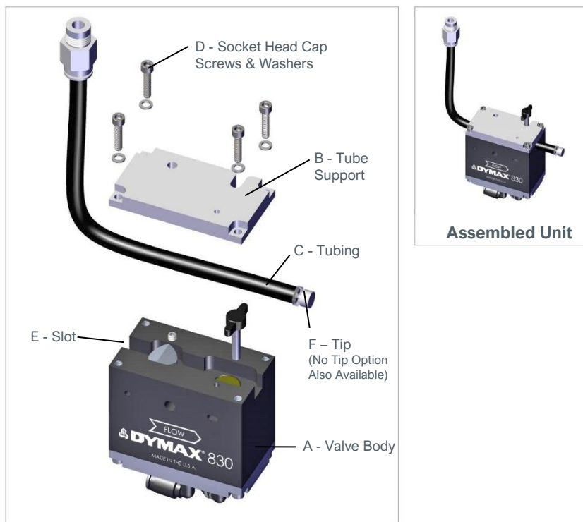
Figure 5. Tubing Installation Procedure
