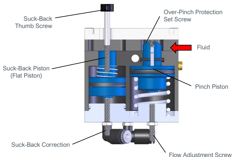
Figure 6. Model 830 Cross Section (Flow from Right to Left)
