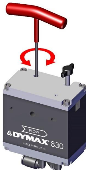
Figure 11. Correcting Over-Pinch Protection
