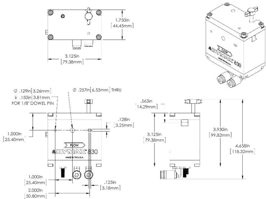
Figure 15. Dimensions
