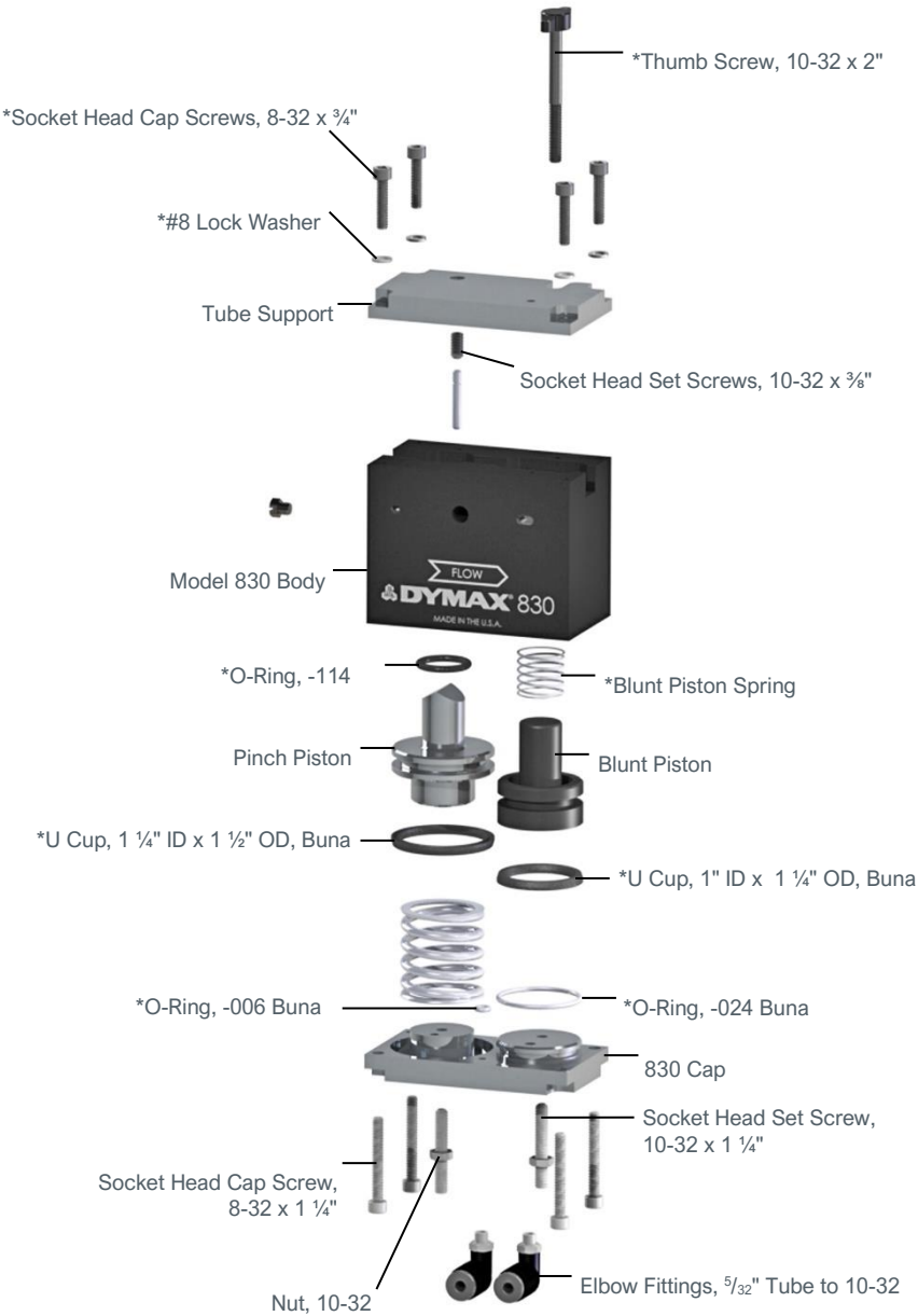
Figure 13. Model 830, Exploded View
