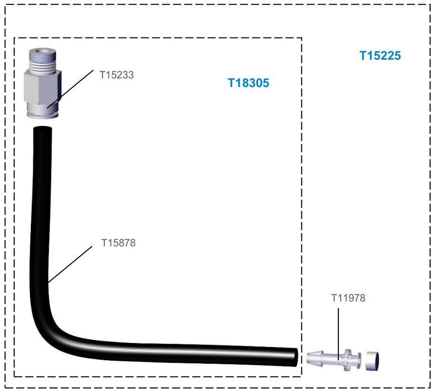
Figure 14. Tubing Assembly
