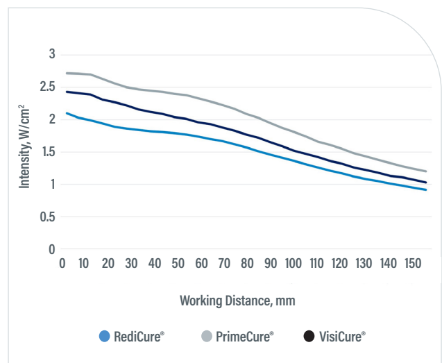
Figure 3. BlueWave® FX-1250 Intensity Over Working Distance
