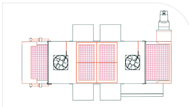
View of SideCure Conveyor (from top) Shown with four 5000-EC lamps side-mounted
