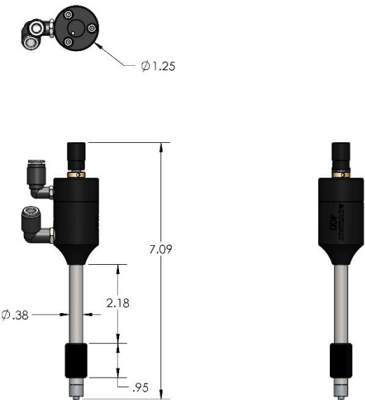
Figure 5. Model 400 Dimensional Drawing
