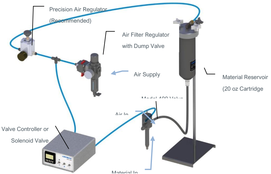
Figure 2. Valve Interconnect Diagram
