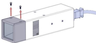
Figure 4. Remove Screws
