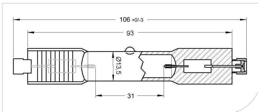
Hg Metal Halide Bulb Dimensions
