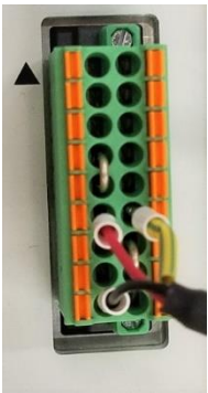
Figure 17. Foot Switch Wiring Pin Locations
