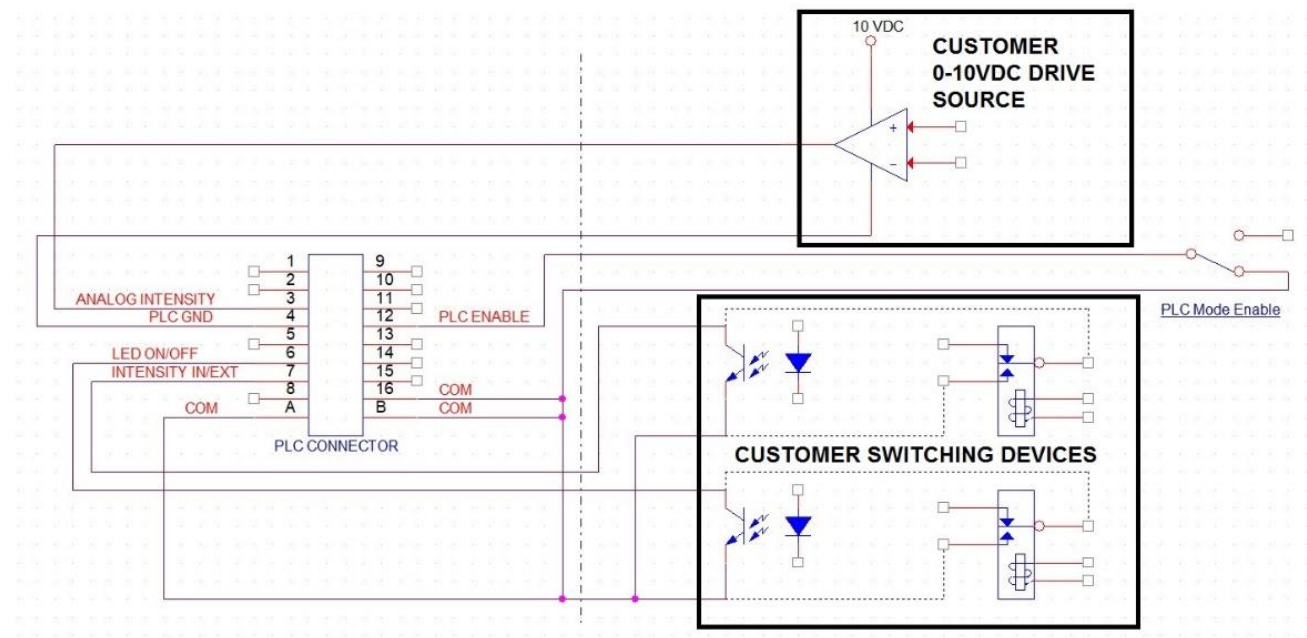
Figure 19. PLC Connection
