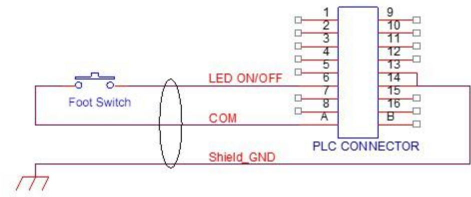
Figure 18. Foot Switch Schematic
