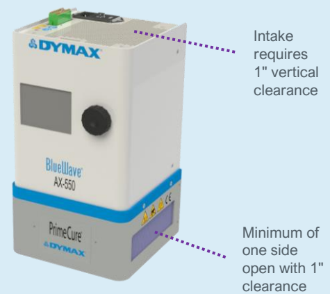
Figure 6. Minimum Clearance
