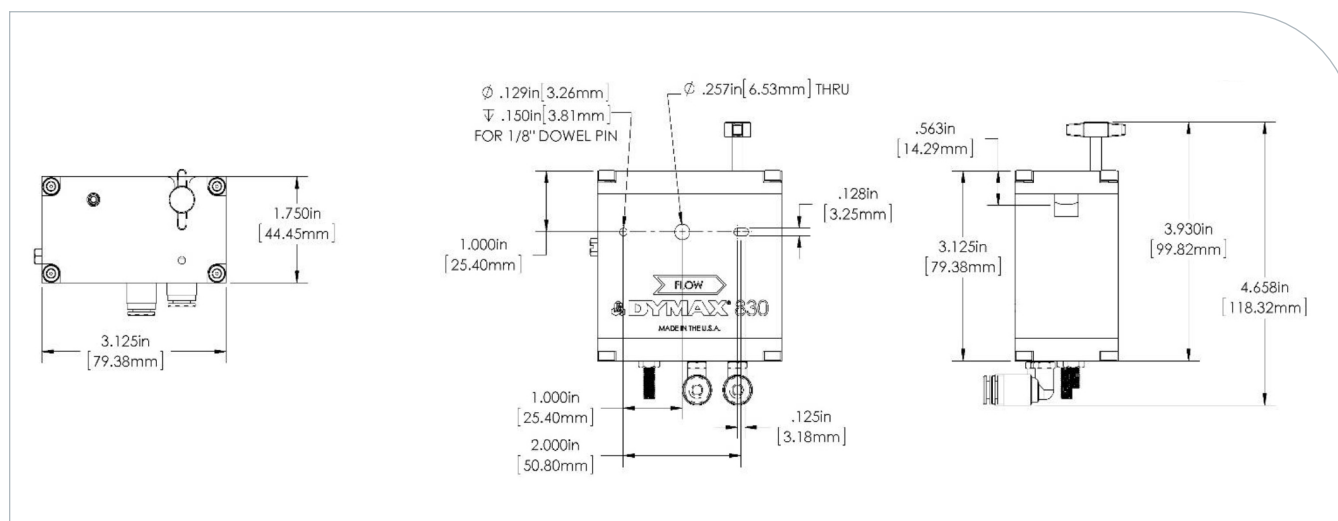
Figure 1. Model 830 Dimensions
