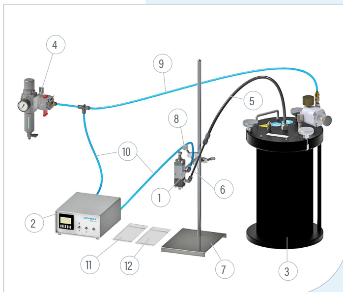
Representative Model 485 Dispensing System (T17734 with Large Bottle Reservoir Shown Below)
