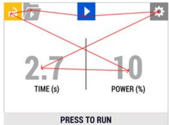
Figure 2. Cursor Path
