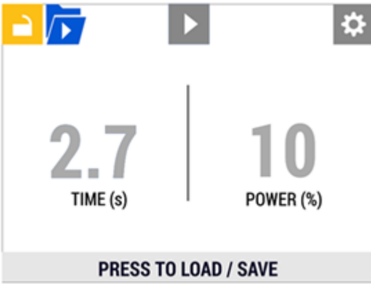
Figure 3. LOAD/SAVE
