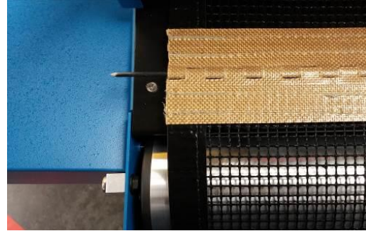
Figure 22. Applying Adhesive
