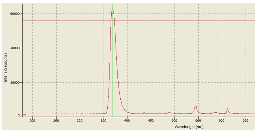
Figure 32. RediCure Wavelength
