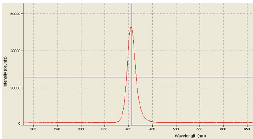
Figure 31. VisiCure Wavelength
