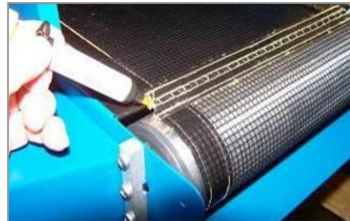
Figure 22. Applying Adhesive
