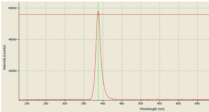
Figure 30. PrimeCure Wavelength
