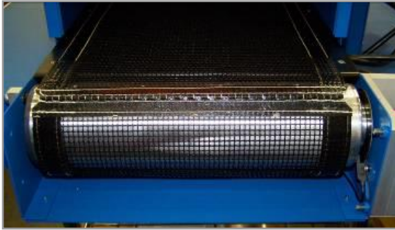
Figure 21. Replacing Belt
